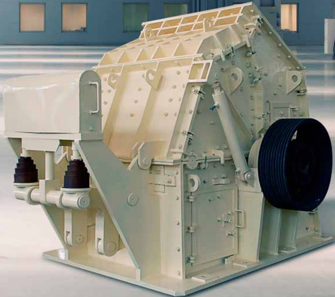
12/12/4 IMPACT CRUSHER
